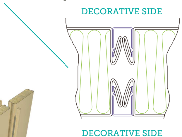
PM-01 Joint panel
